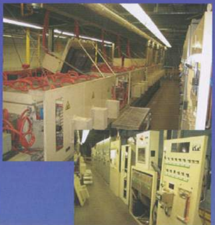
J878.14- Harper 1520C high temperature pusher type sintering furnace.
