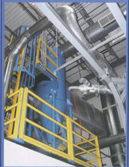
J878.12- Separator manufactured by Sly as Model CBR-35-196, S/N 0039, manufactured 3-2007.
